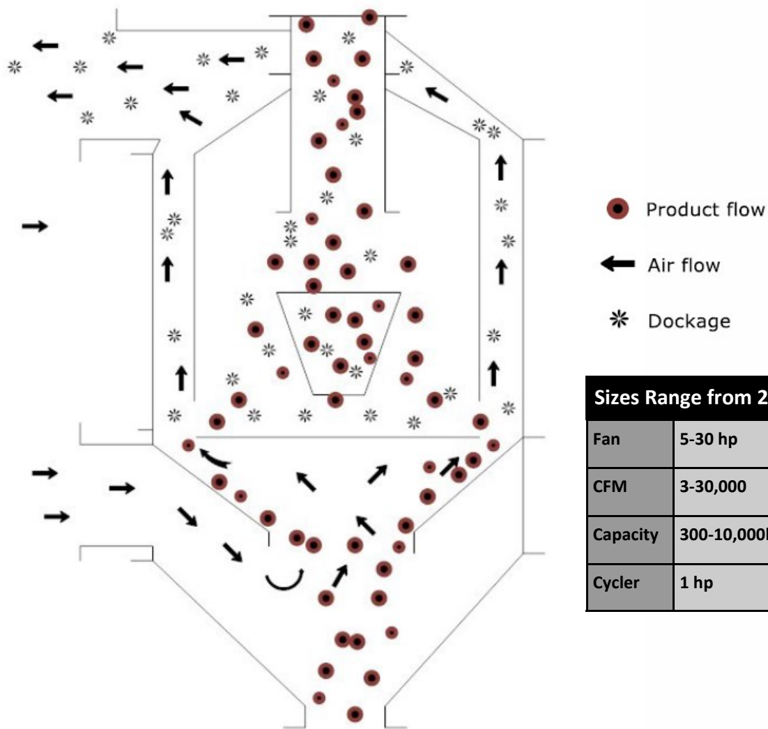
Cyclo Aspirator Flow Diagram
